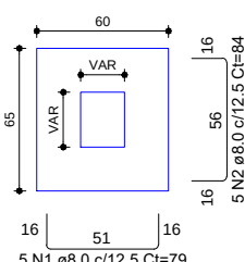
S2=S4=S7=S8=S10=S11= S12=S13=S15=S16=S19 PLANTA ESC 1:25
